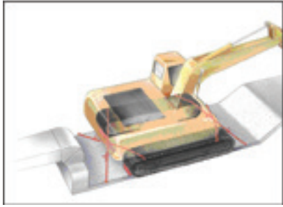
Figur 37: Diagonal surring
