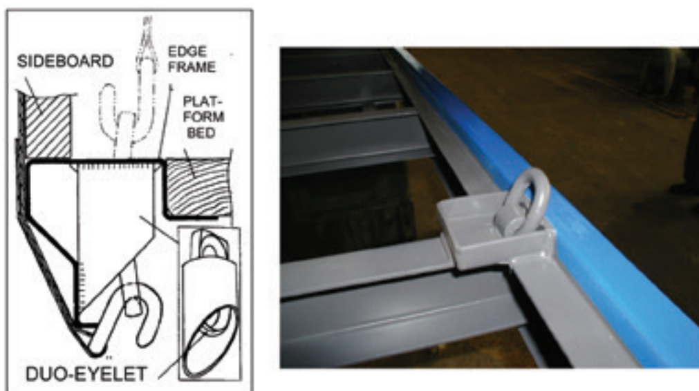
Figur 12: Surringsøsken
